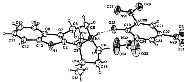
Figure 4. ORTEP drawing of cis - 17 •picric acid. Displacement ellipsoids are shown at the 30% probability level.
