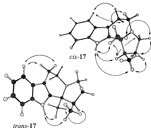
Figure 5. Observed NOE effects on cis - and trans -17.
