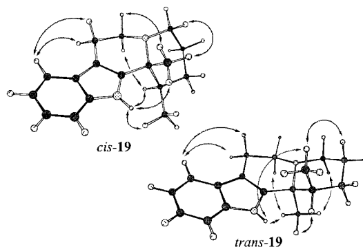
Figure 7. Observed NOE effects on cis - and trans -19.
