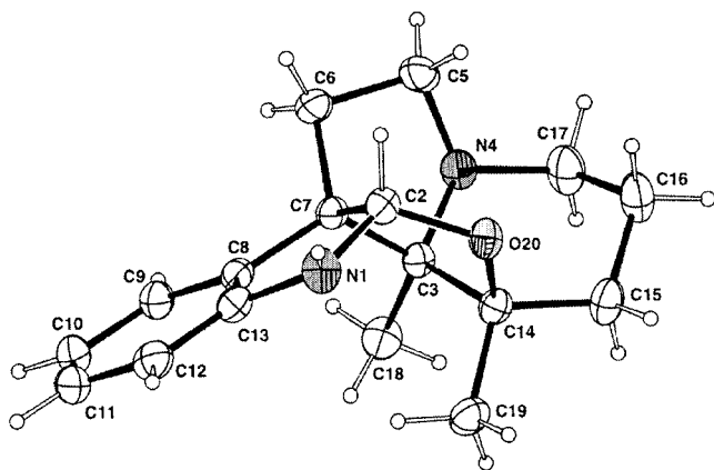
Figure 2. ORTEP drawing of 22 . Displacement ellipsoids are shown at the 30% probability level.
