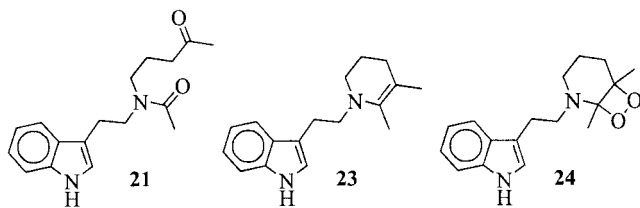
Figure 3. Ketone 21 and putative intermediates 23 and 24 .
