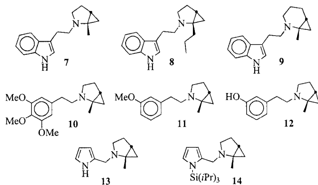
Figure 1. Aminocyclopropanes 7 – 14 .
