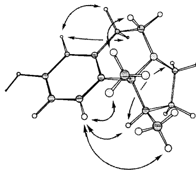
Figure 8. Observed NOE effects on cis - 20 .
