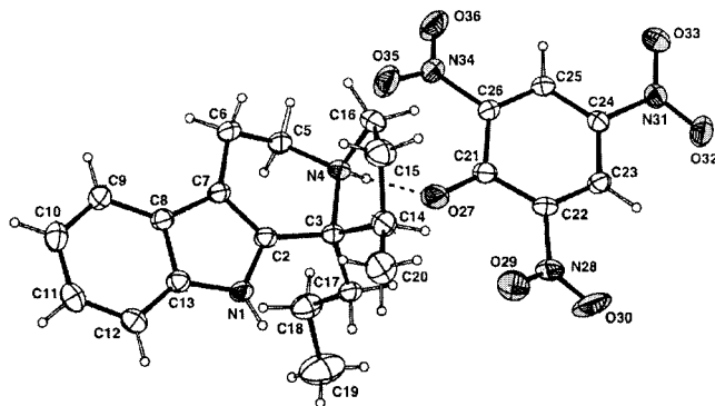
Figure 6. ORTEP drawing of 18 •picric acid. Displacement ellipsoids are shown at the 30% probability level.
